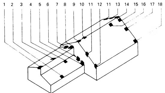
9 Shaped tiles
